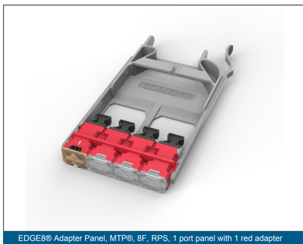
EDGE8® Adapter Panel, MTP®, 8F, RPS, 1 port panel with 1 red adapter
